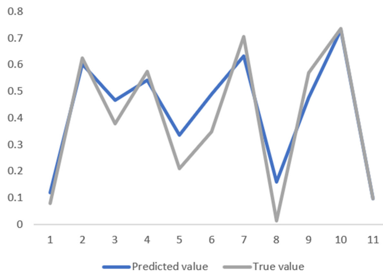
Figure 7. Comparison between the predicted value and the real value of the training data of 6 eigenvalues of CatBoost algorithm
