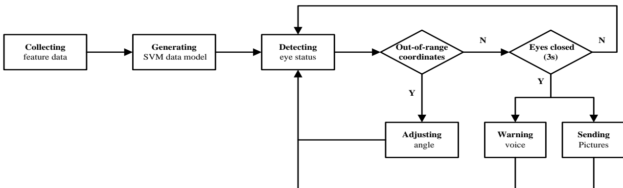
Fig. 2 Flow chart of eye fatigue state detection algorithm
