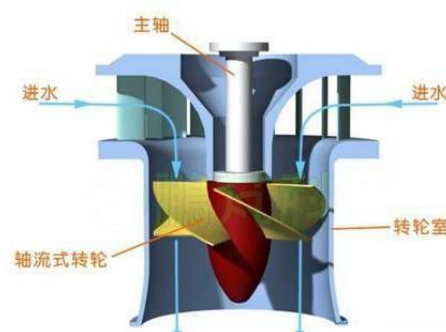
Fig. 2 Axial flow impeller structure
